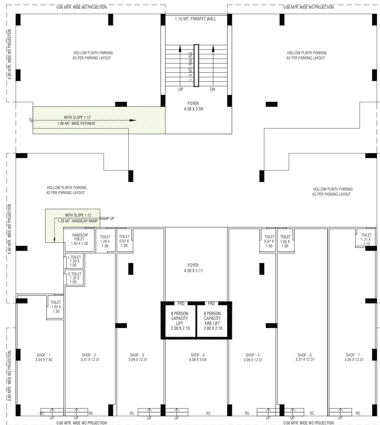
GROUND FLOOR PLAN ( PART H.P. & PART S.P. )
